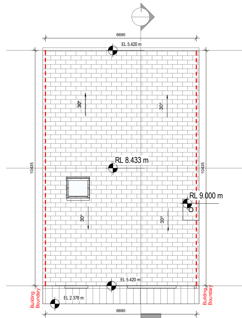
3 Roof Plan 1 : 100 @ A3
