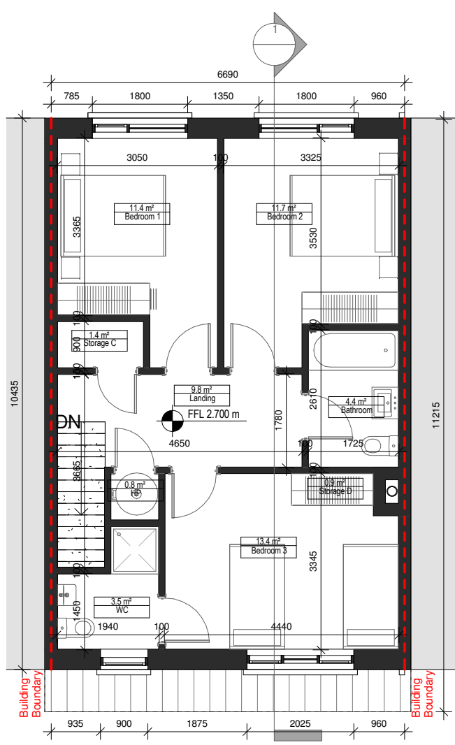
2 First Floor Plan 1 : 100 @ A3
