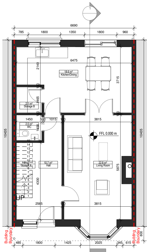
1 Ground Floor Plan 1 : 100 @ A3
